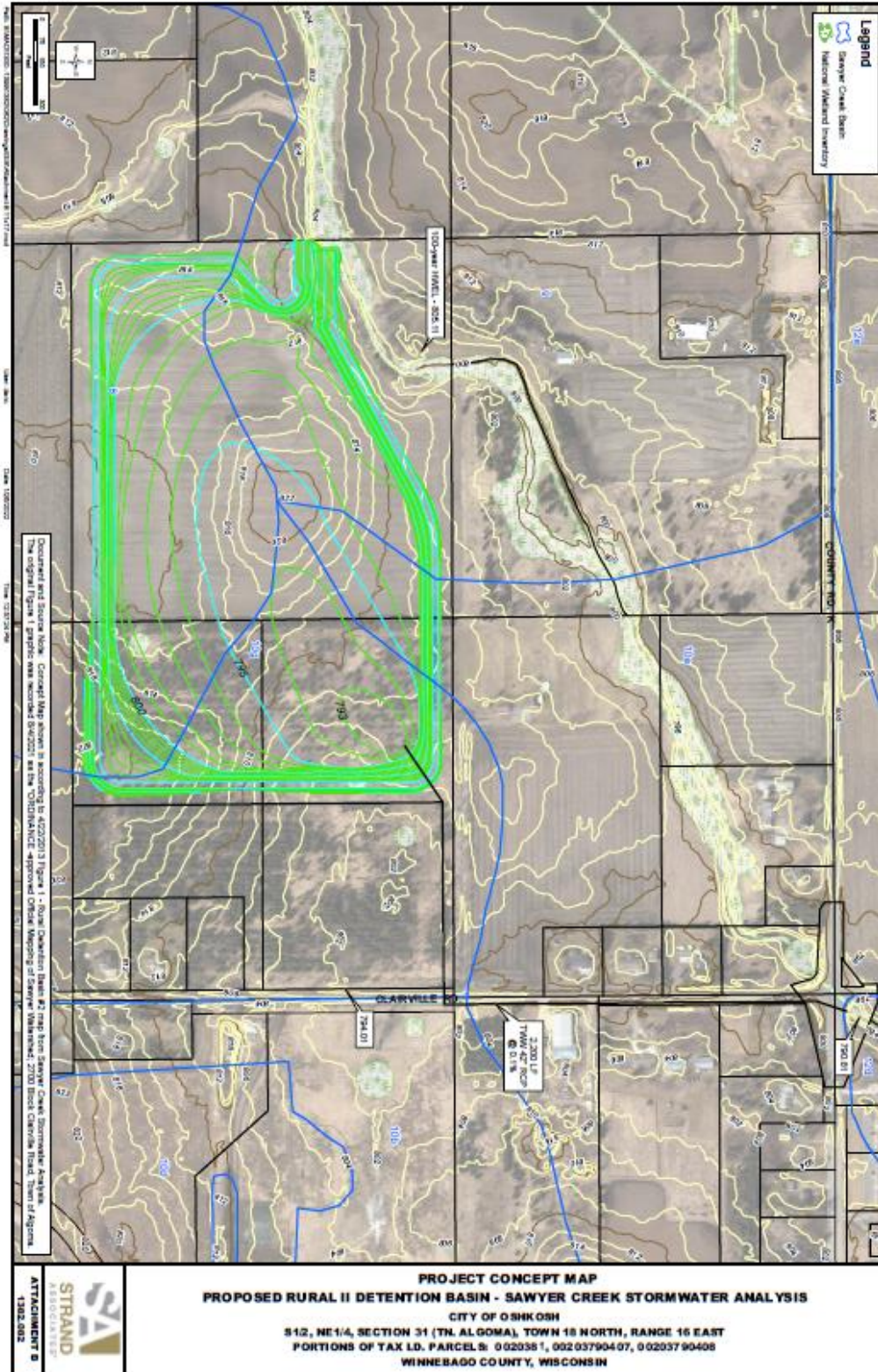
Figure 1: The proposed design of the Oshkosh Rural II Detention Basin in the Town of Algoma, Winnebago County, WI (DATCP, 2023a).
